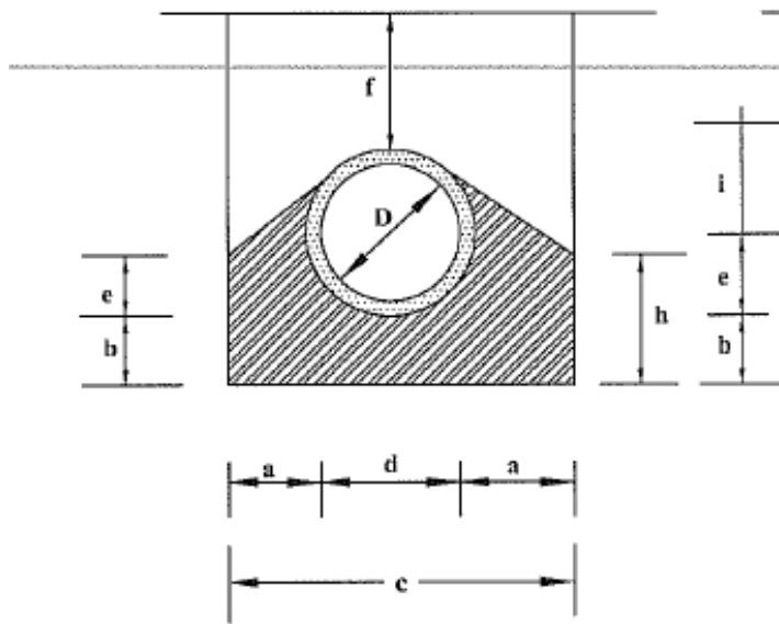
PROFILE III (CONCRETE)
