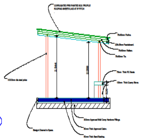
Section x-x
